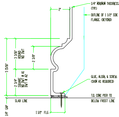
BASE DETAIL
