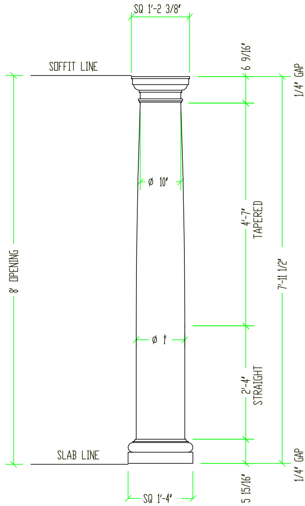
COLUMN COVER ELEVATION
