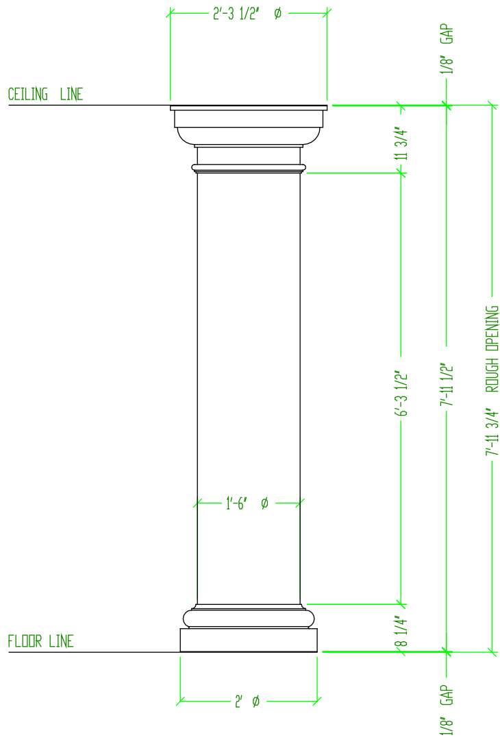
COLUMN COVER ELEVATION
