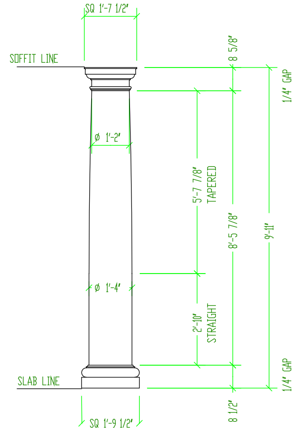
COLUMN COVER ELEVATION
