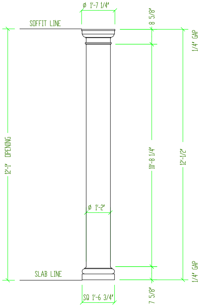
COLUMN COVER ELEVATION
